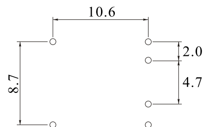
Land pattern
